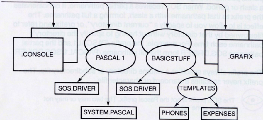
Figure 4-9. Pathnames
