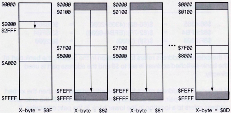
Figure 2-10. Increment Path
