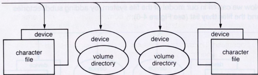
Figure 4-5. Top-Level Files
