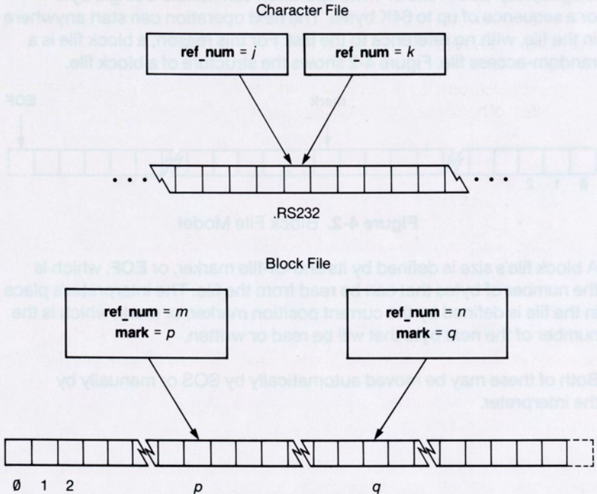
Figure 4-3. Open Files
